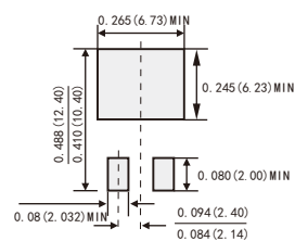
( TO-252 )
