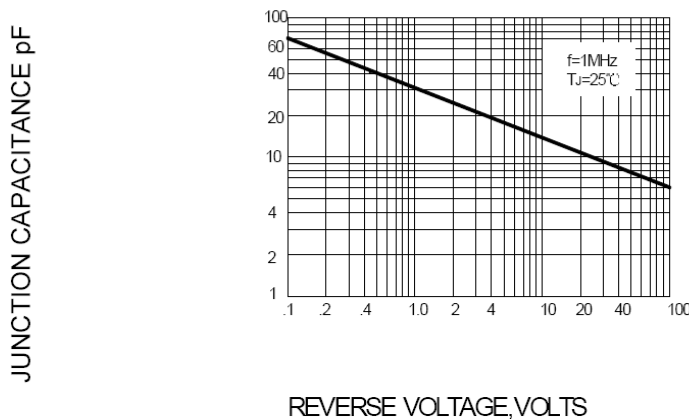
FIG.5-TYPICAL JUNCTION CAPACITANCE
